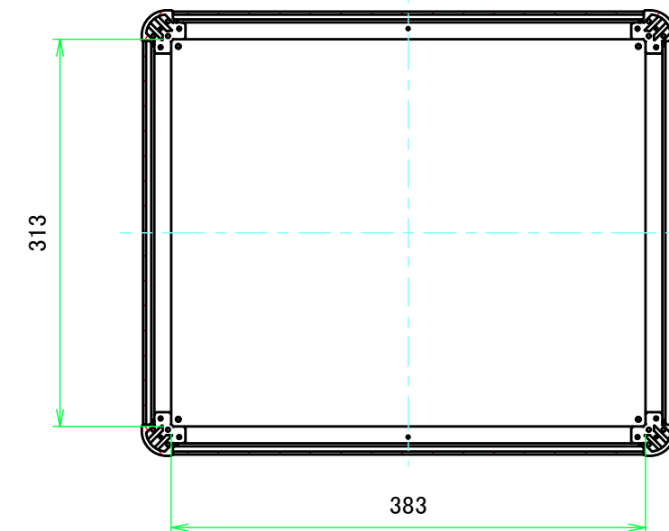
C-C (1:5.5)
